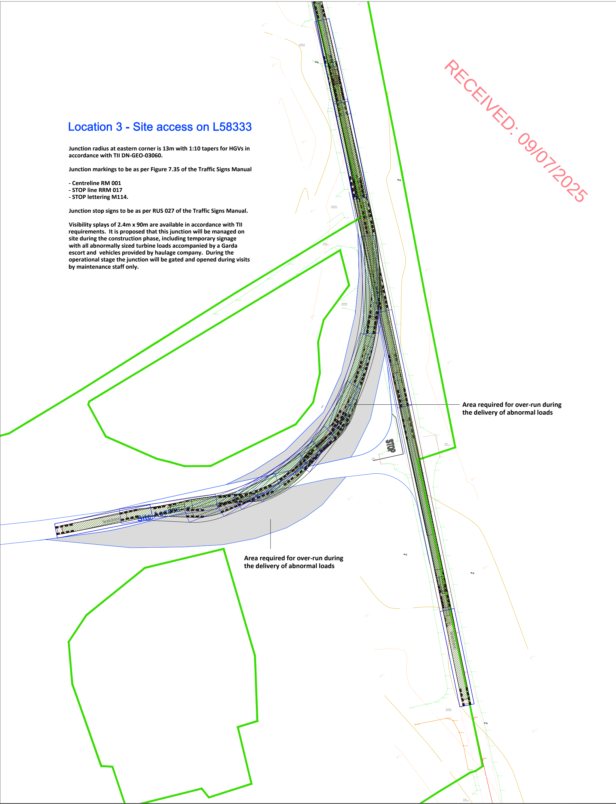
Figure 15-14 Location 3 - Access junction on L58333, autotrack assessment, tower extended artic
