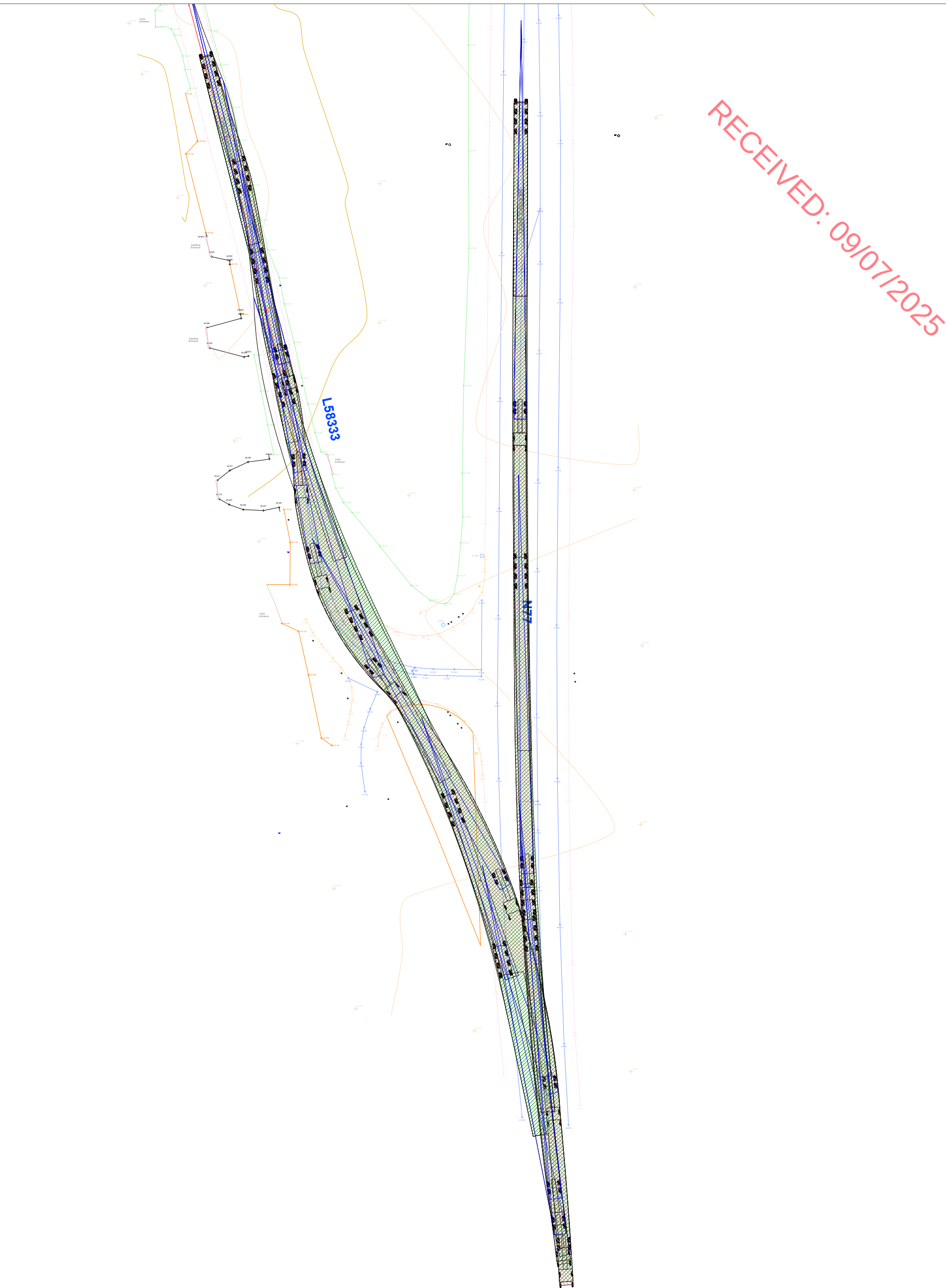
Figure 15-9 Location 2 - N77 / L58333, autotrack assessment, blade extended artic
