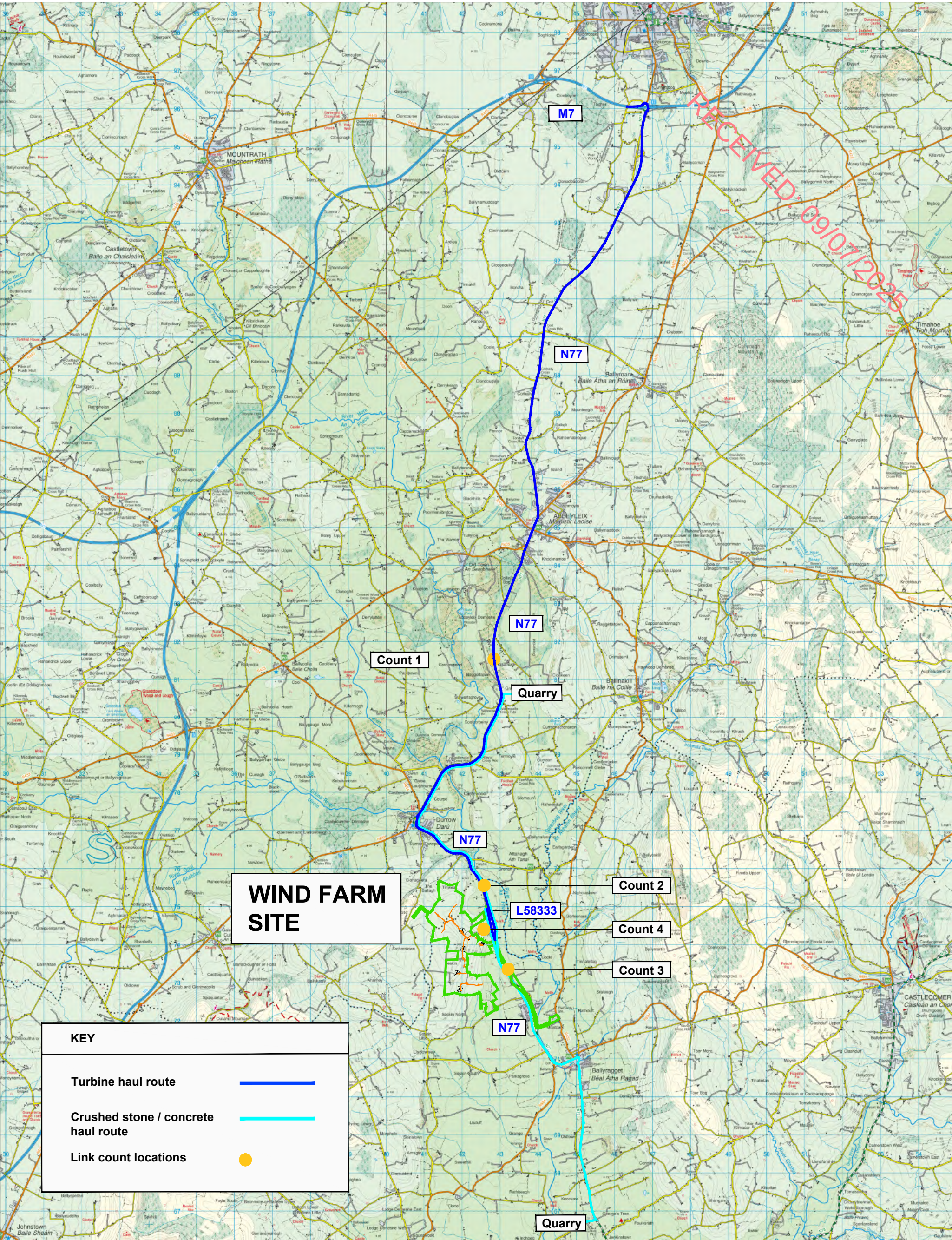
Figure 15-2b Link count locations
